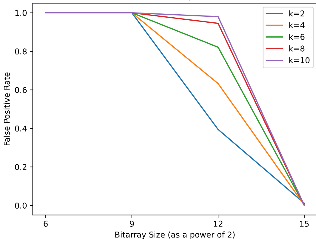
False Positive Rate Analysis on "can" Task
